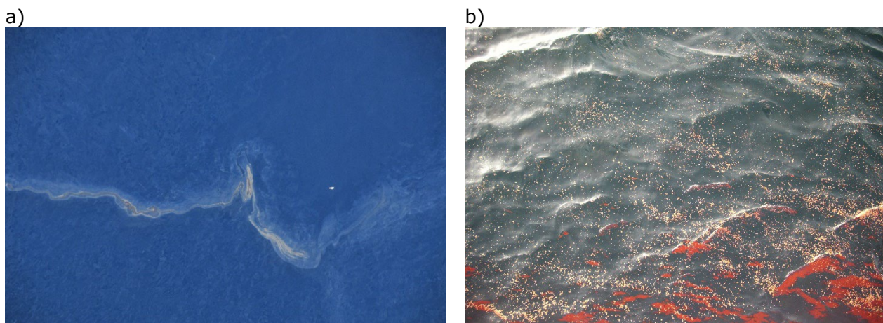
Figure 7 a): 2018 image - Release resulting from a processing upset, cold process fluid destabilised production chain increasing the concentration of oil in produced water. b): 2012 image - Mix of drilling fluids along with condensate, it was releasing new and old drill fluids which would likely include base oil and drilling chemicals as well as condensate.
